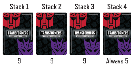
Stack Sizes for a 2-player game.
